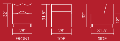
WAVE BACK CHAIR #9175-AL5
